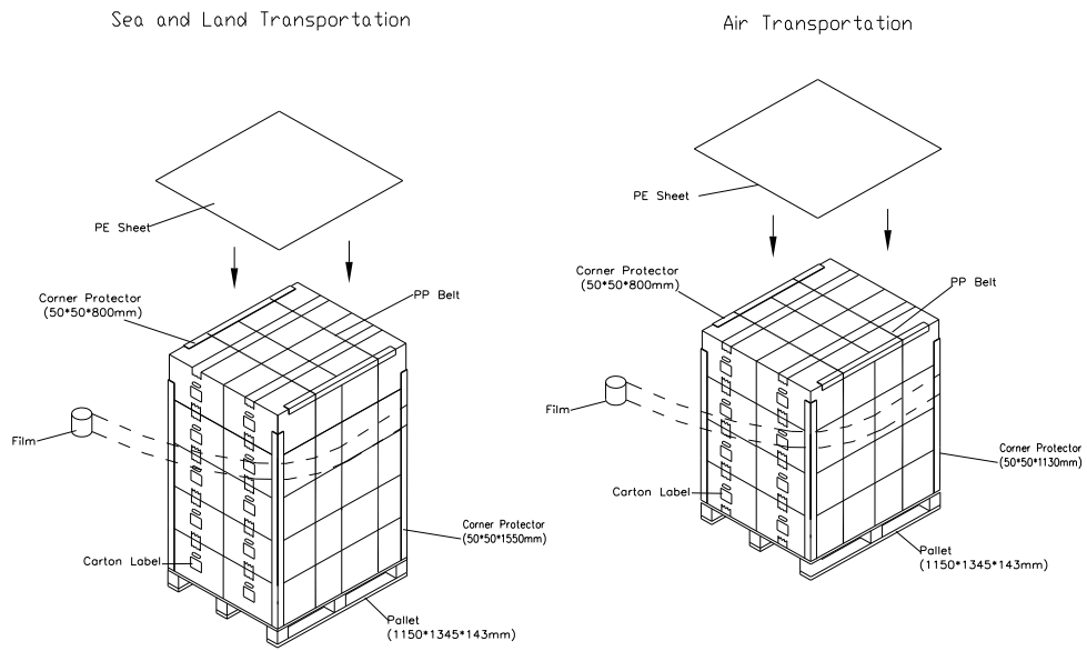
Figure. 8-2 Packing method
